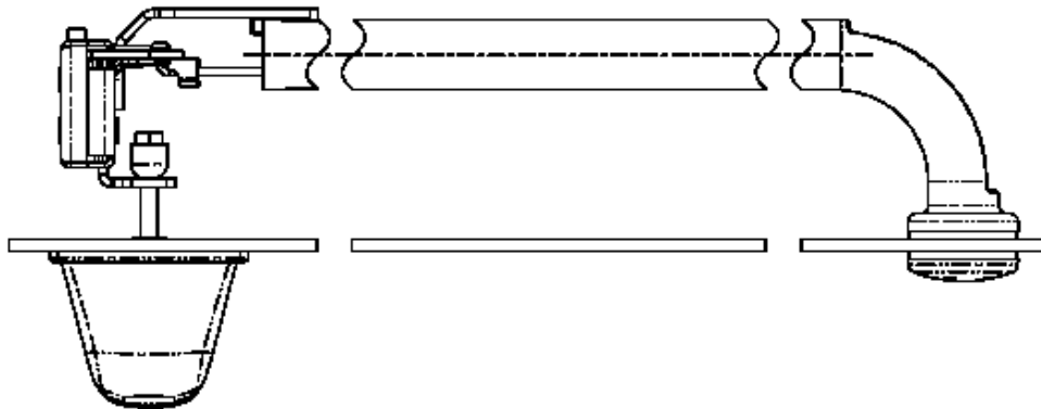
Typical System Drawing With TriMark 020-0800 Pull Handle
